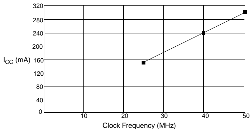
Figure 11. Typical I CC Versus Frequency
