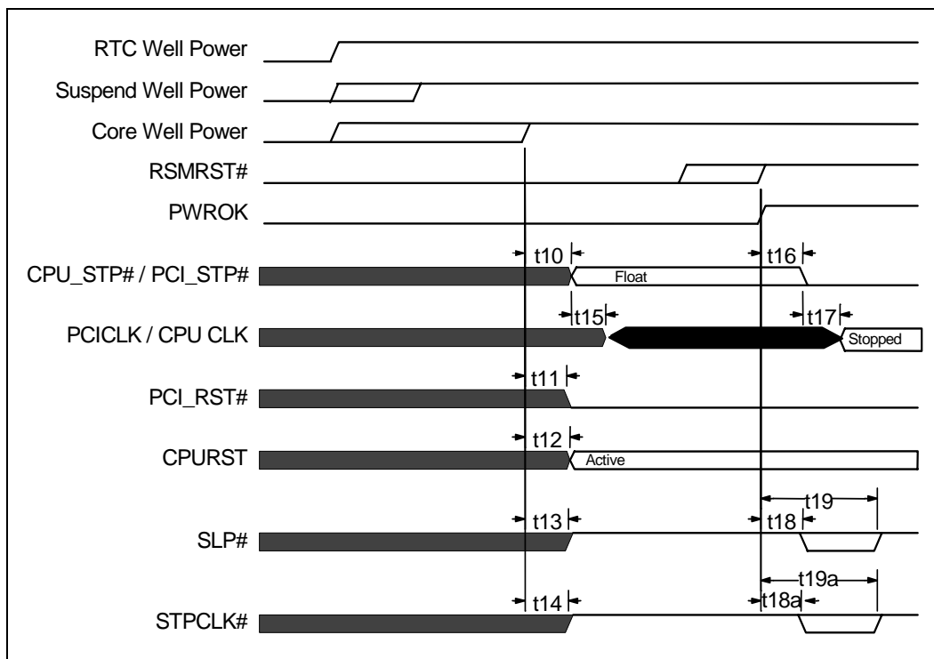
Figure 25. Core Well Power and PWROK Activated Signals (Core Well Power Applied before RSMRST# Inactive)
