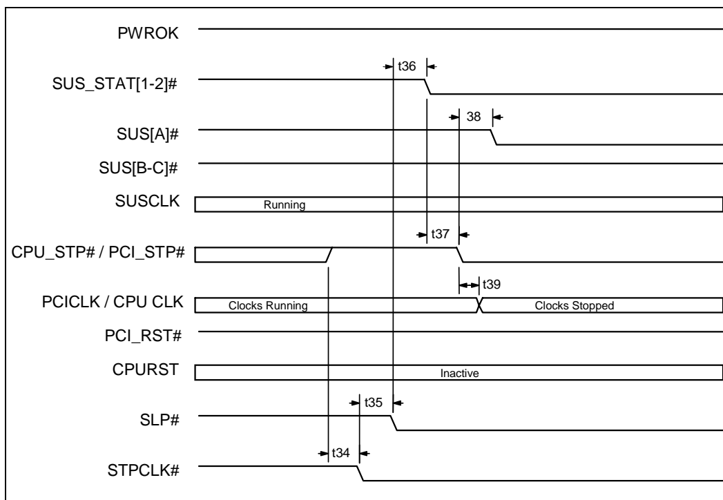
Figure 27. On to POS
