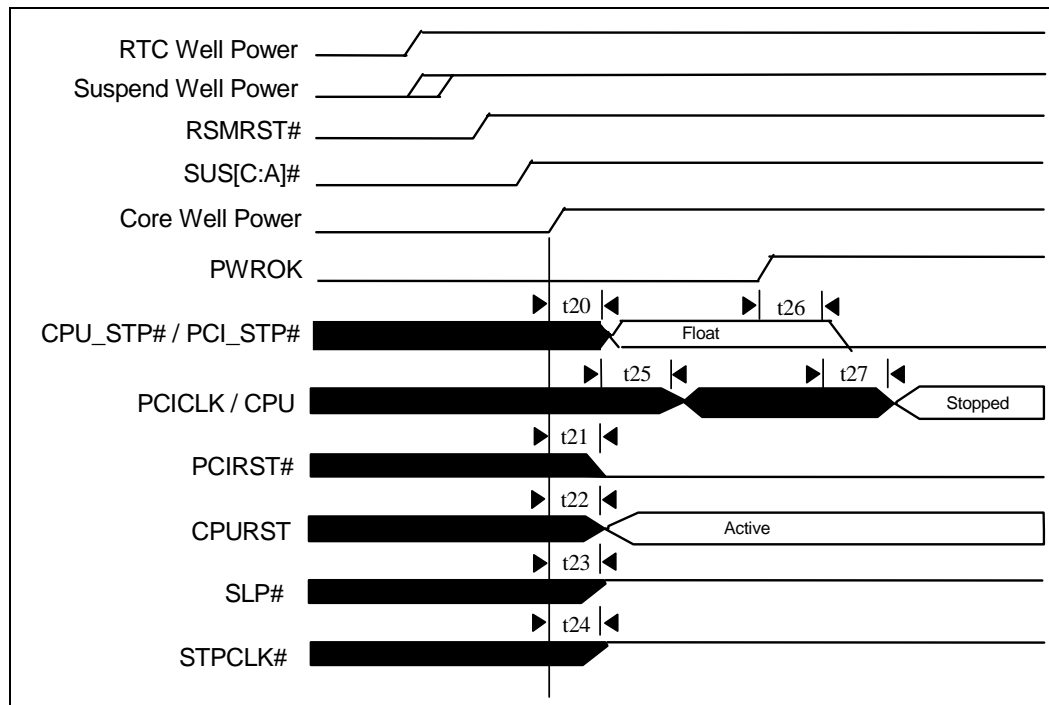
Figure 24. Core Well Power and PWROK Activated Signals (RSMRST# Inactive before Core Well Power Applied)
