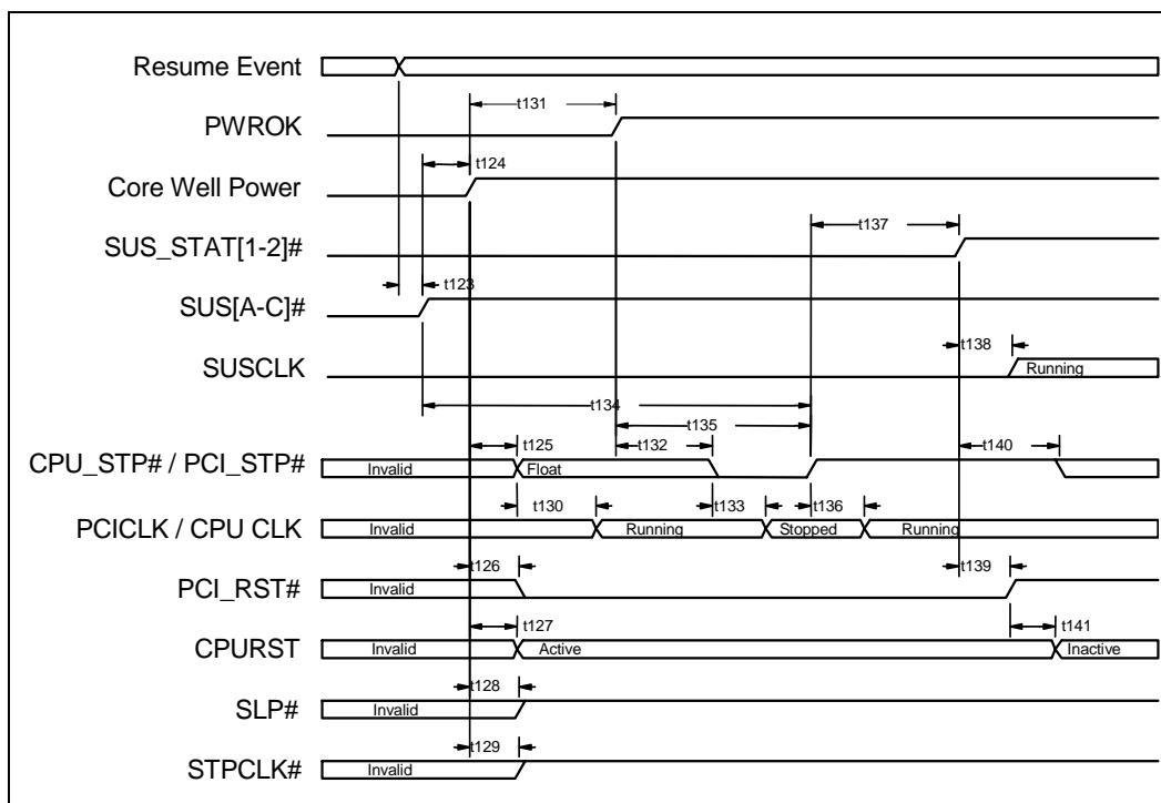
Figure 34. STD/SOff to On
