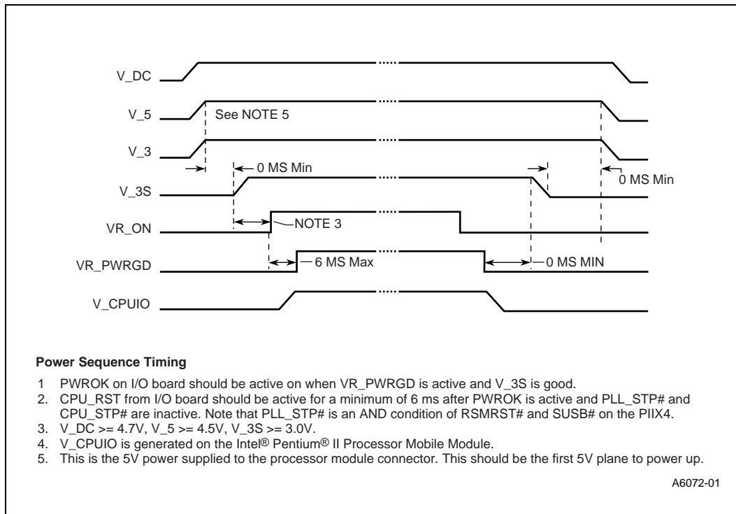
Figure 41. Power On Sequence
