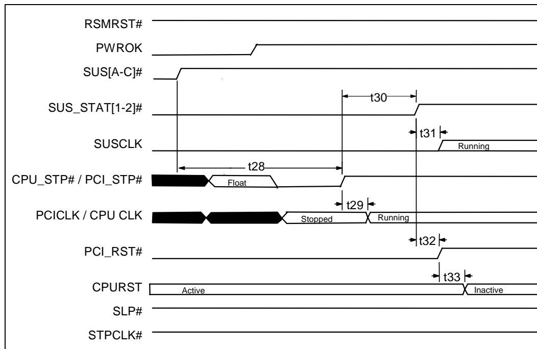
Figure 26. Mechanical Off to On
