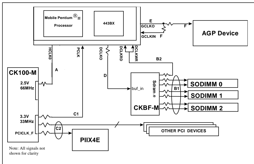
Figure 12. EMC-2 Clocking Layout
