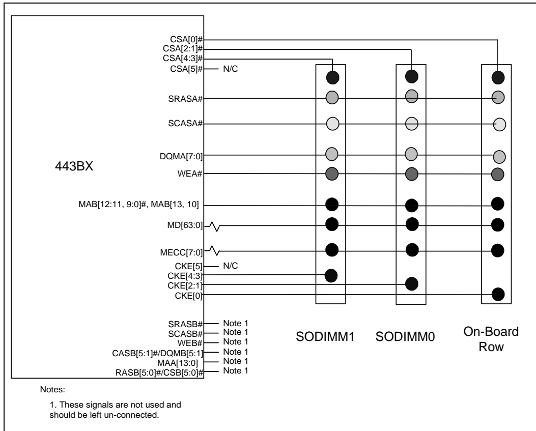
Figure 5. SDRAM - One On-board Bank, Two SODIMMs
