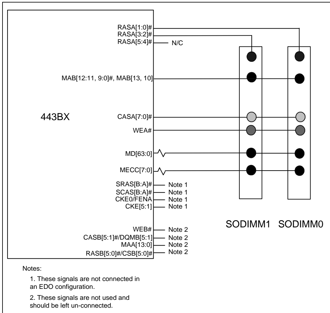
Figure 3. EDO DRAM - Two SODIMMs
