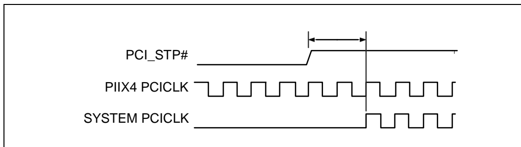
Figure 23. PCI Clock Start Timing
