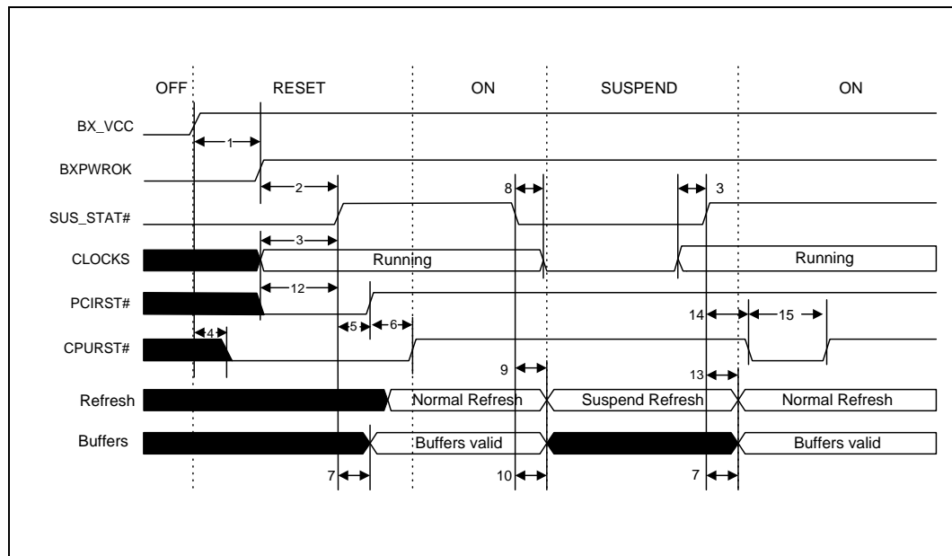
Figure 39. Suspend/Resume with Inactive PCIRST and Active CPURST#
