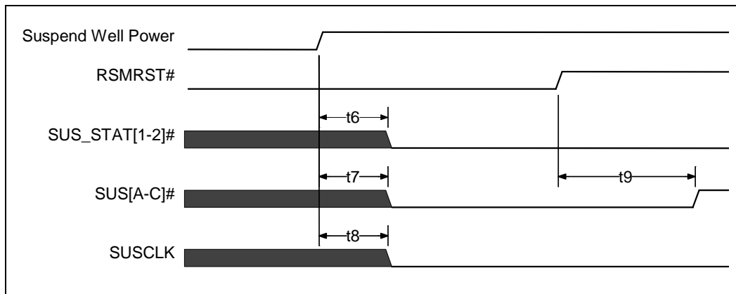
Figure 21. Suspend Well Power and RSMRST# Activated Signals
