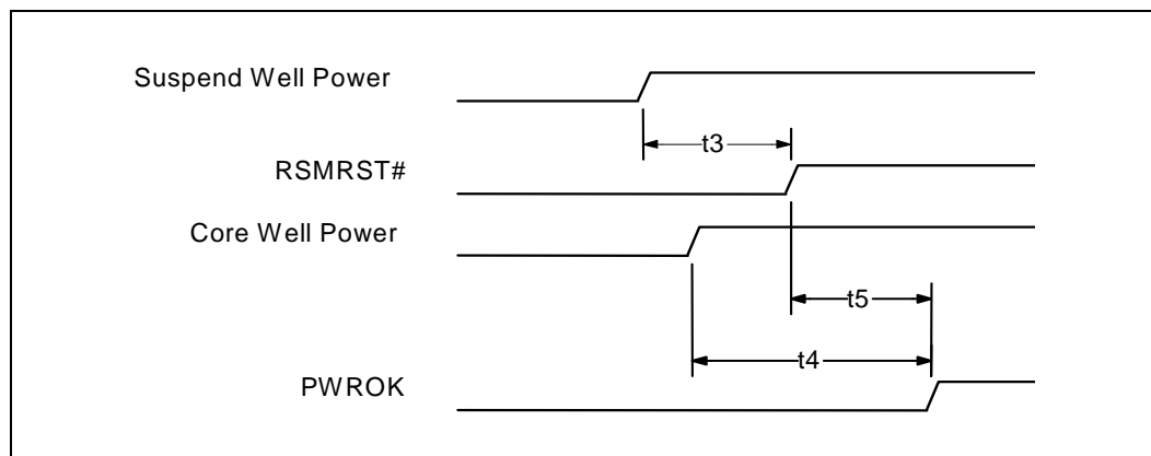
Figure 20. RSMRST# and PWROK Timings
