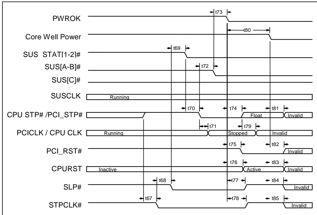
Figure 31. On to STR
