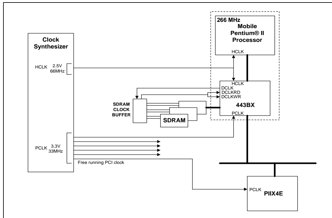
Figure 8. Clock Connections to the EMC-2 Module
