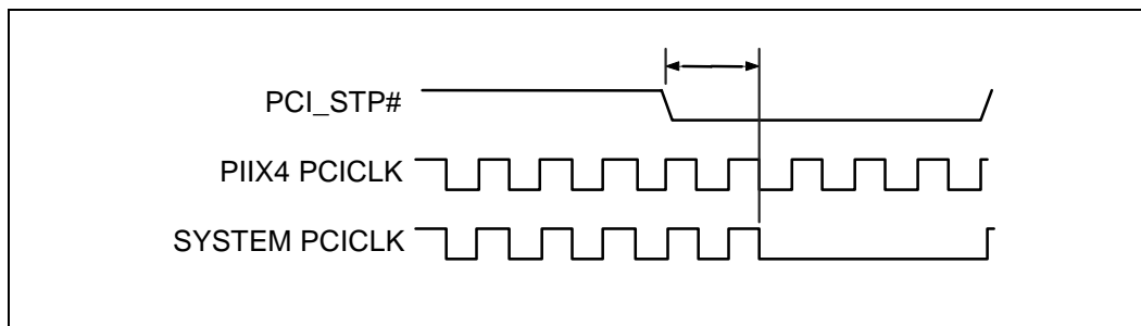
Figure 22. PCI Clock Stop Timing
