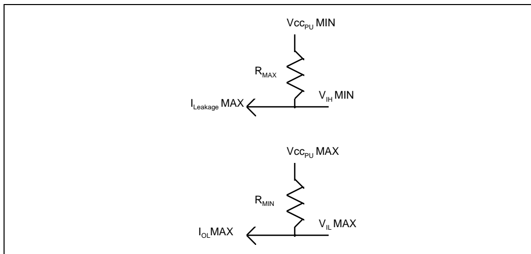
Figure 16. Pull-up Resistor Example
