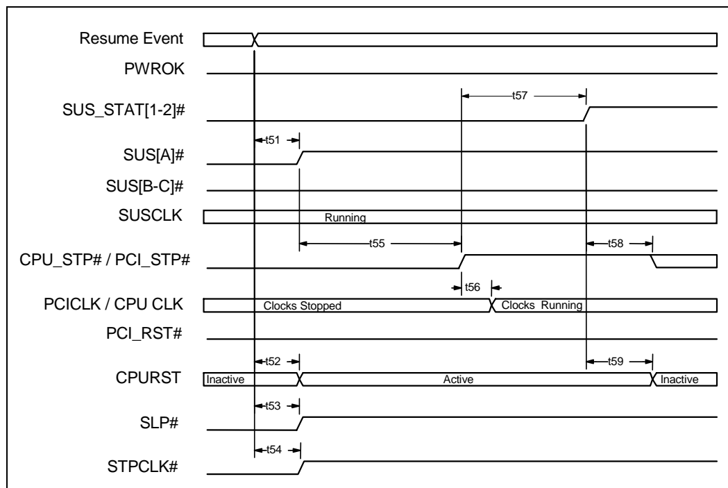
Figure 29. POS to On (with Processor Reset)
