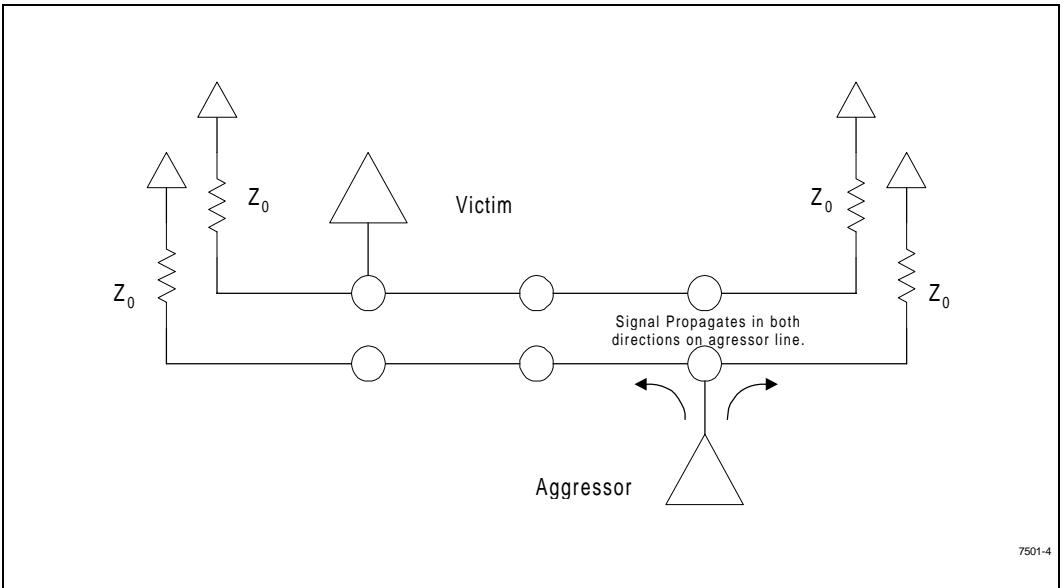
Figure 4. Aggressor and Victim Networks
