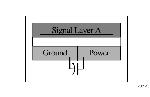
Figure 10. One Layer with Multiple Reference Planes
