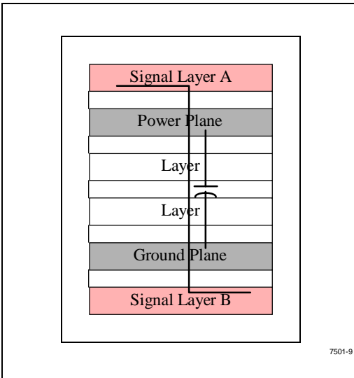
Figure 9. Layer Switch with Multiple Reference Planes
