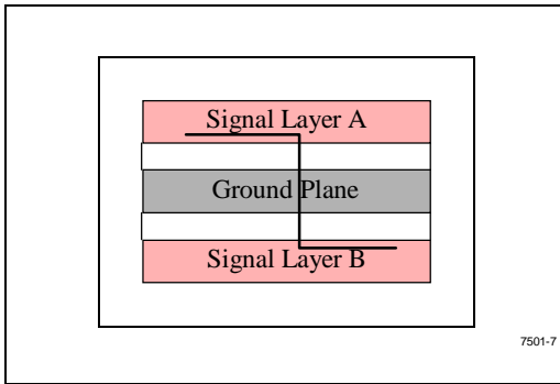
Figure 7. Layer Switch with One Reference Plane
