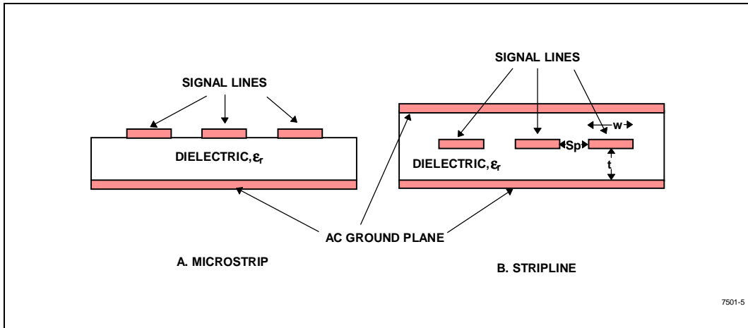
Figure 5. Transmission Line Geometry: (A) Microstrip (B) Stripline
