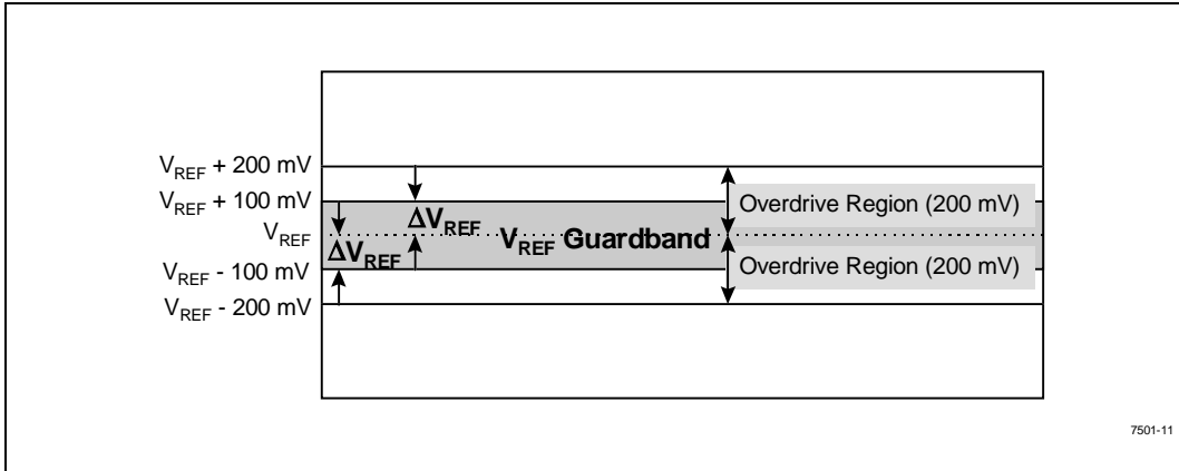
Figure 11. Overdrive Region and VREF Guardband
