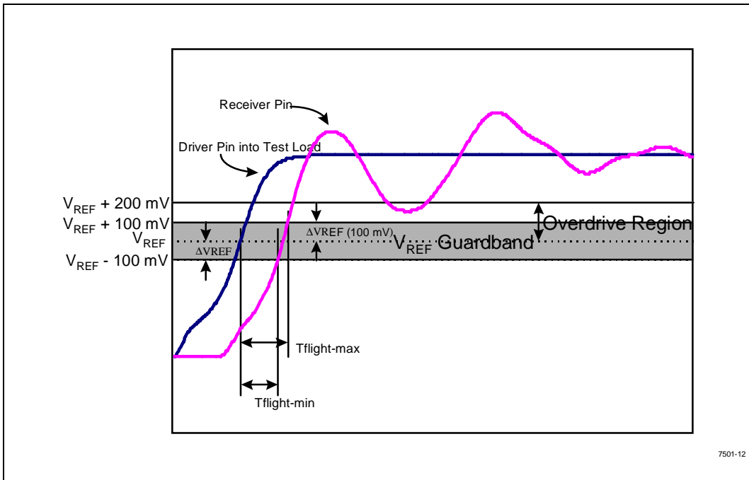
Figure 12. Rising Edge Flight Time Measurement
