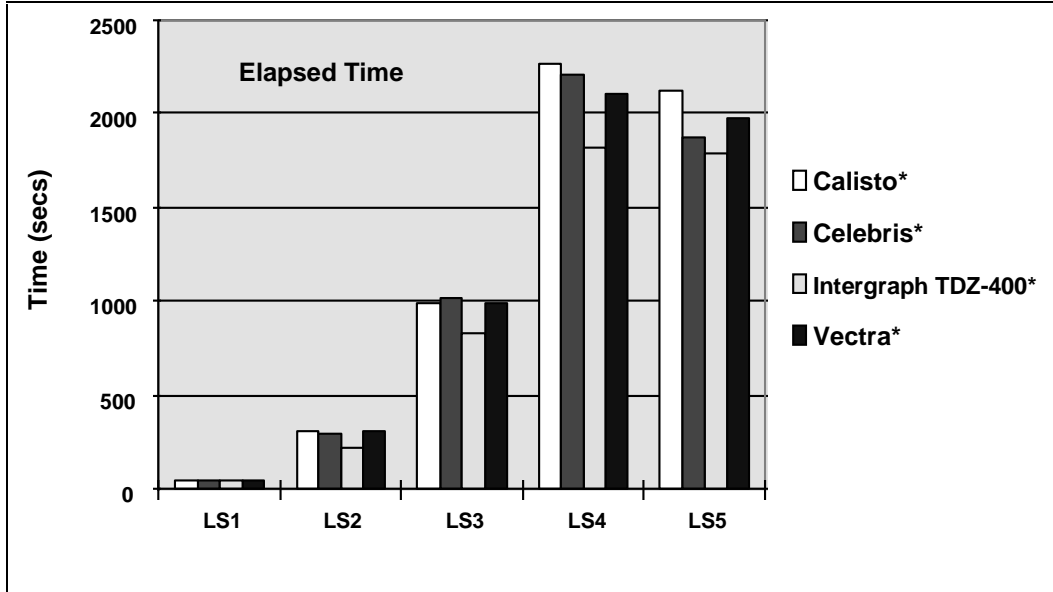
Figure 13. ANSYS* Performance
