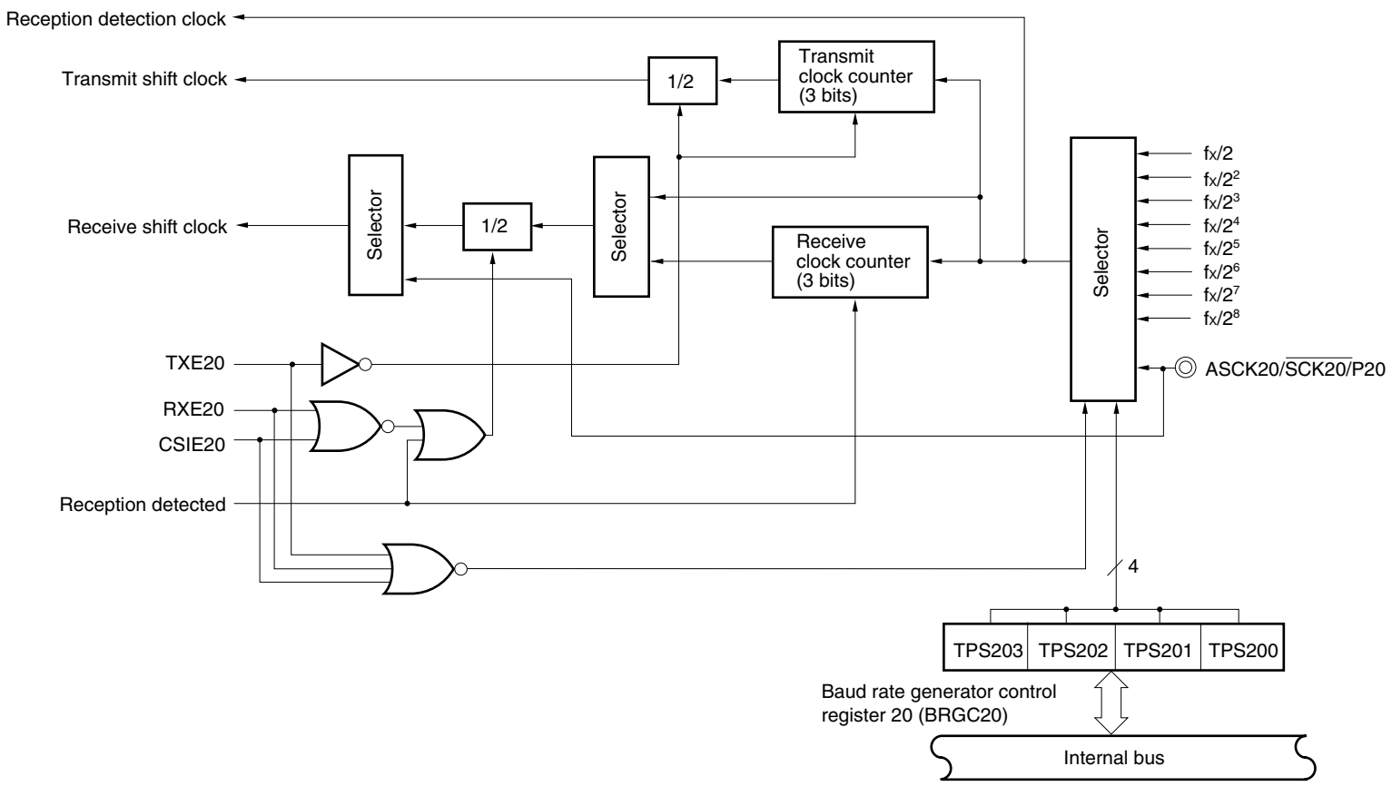
Figure 9-2. Block Diagram of Baud Rate Generator 20
