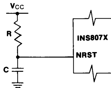
FIGURE 8. Reset Implementation
