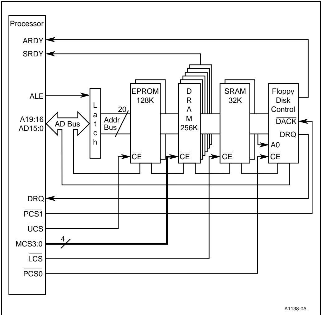
Figure 6-13. Typical System
