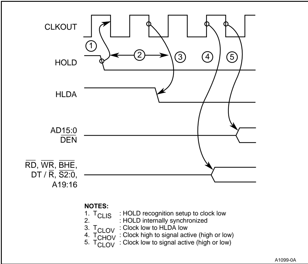
Figure 3-38. Exiting HOLD
