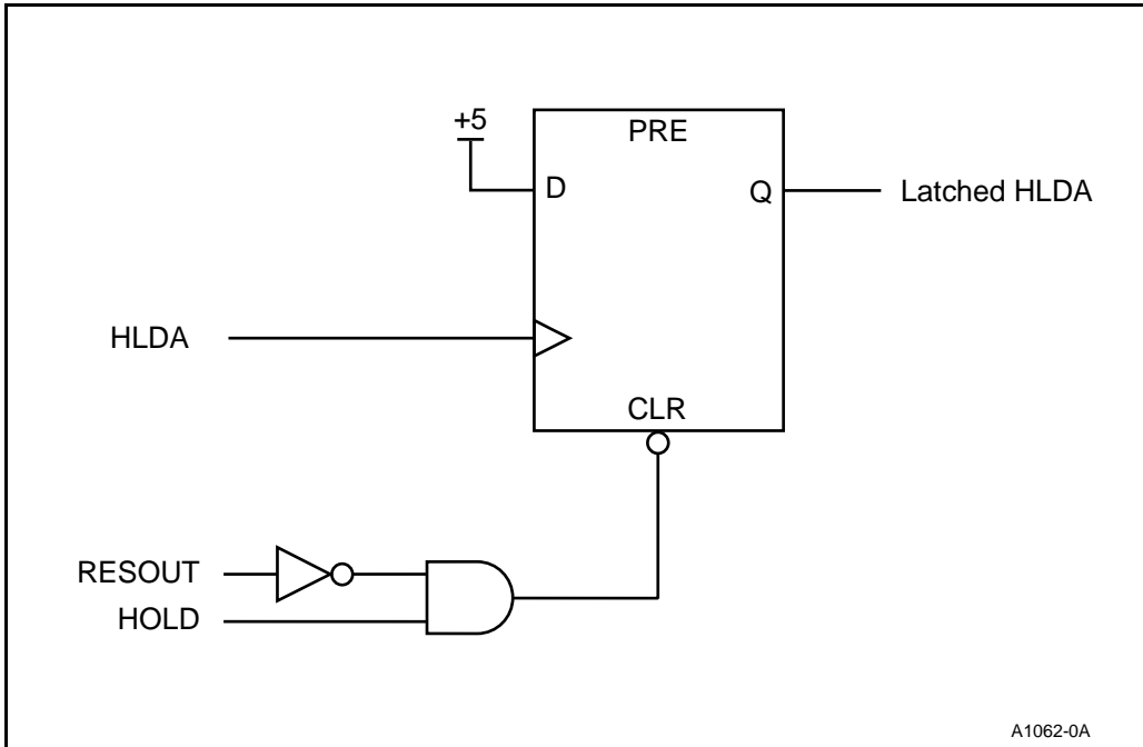
Figure 3-37. Latching HLDA
